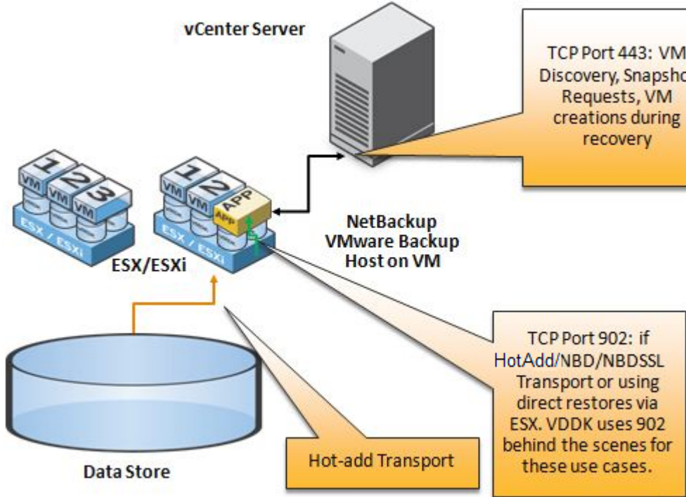
Figure 3-4 VMware ports
